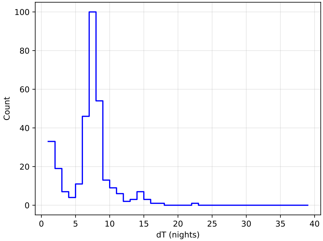
Imc_filter_balance_v3.4_10yrs all bands: DD:EDFS Delta Nights Histogram
