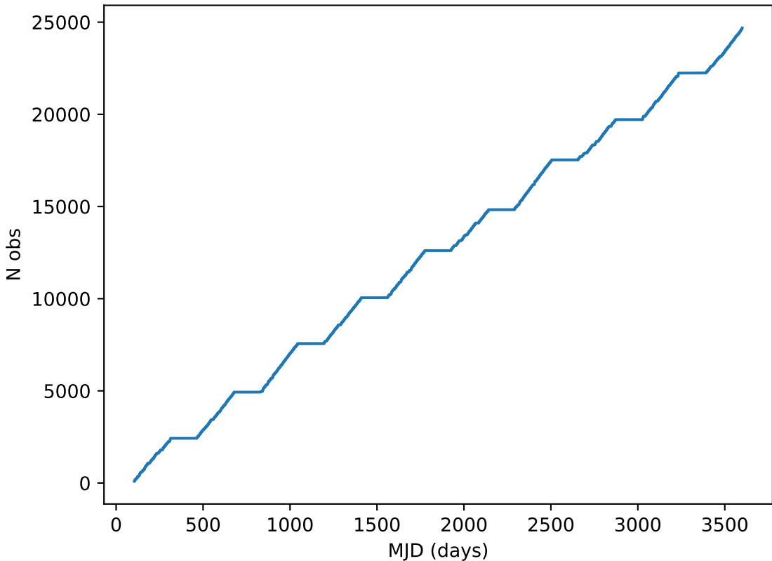
Imc_filter_balance_v3.4_10yrs all bands: DD:EDFS Cumulative NVisits
