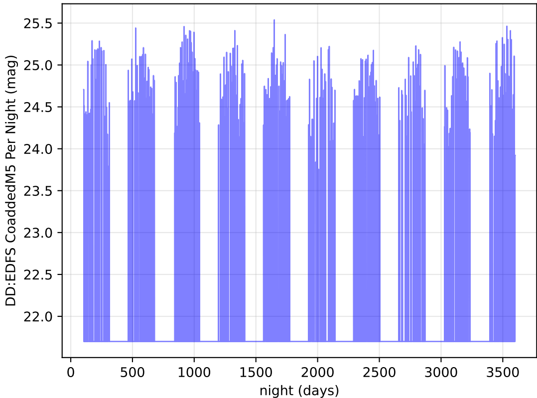
Imc_filter_balance_v3.4_10yrs z band: DD:EDFS CoaddedM5 Per Night
