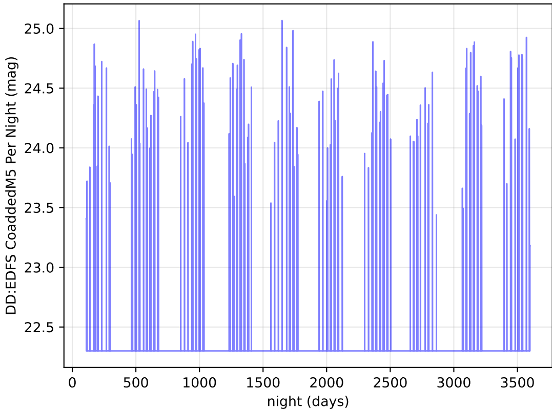
Imc_filter_balance_v3.4_10yrs u band: DD:EDFS CoaddedM5 Per Night
