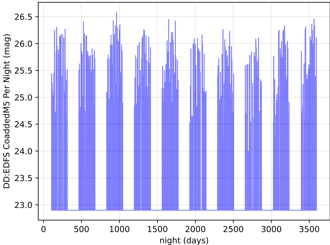
Imc_filter_balance_v3.4_10yrs r band: DD:EDFS CoaddedM5 Per Night
