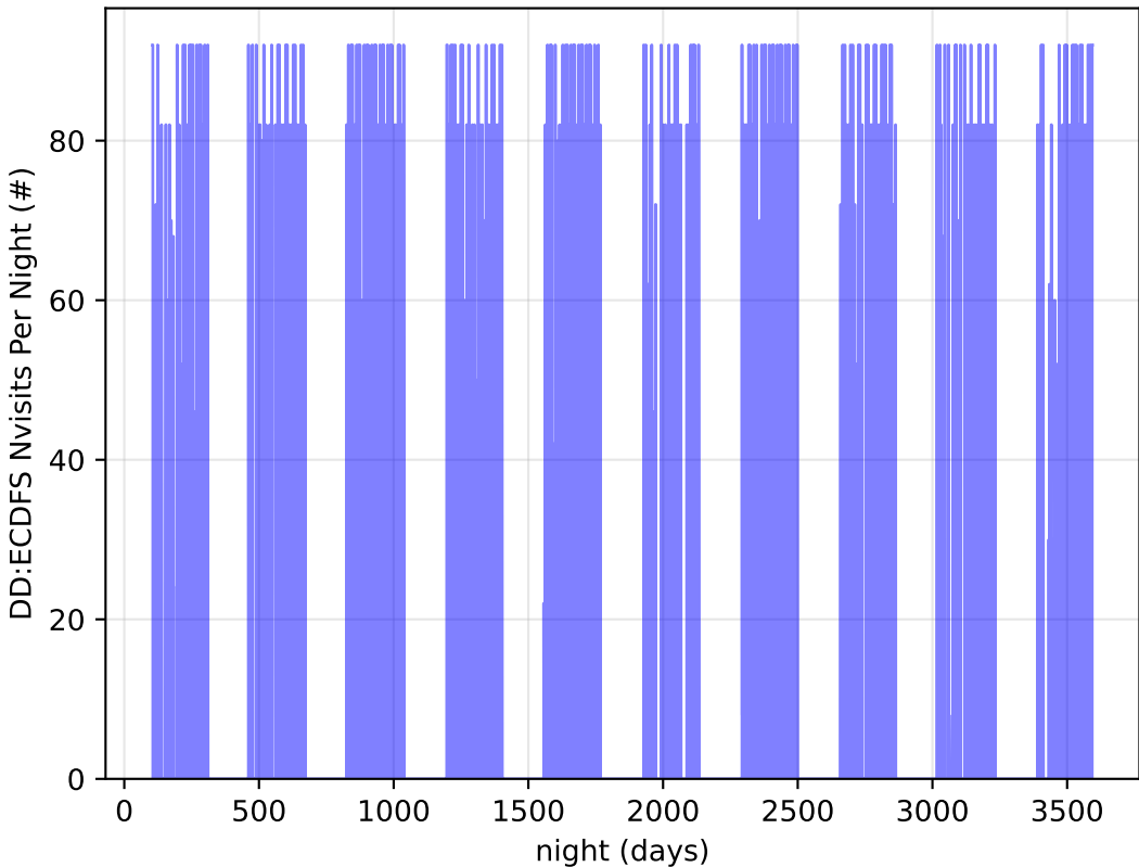
Imc_filter_balance_v3.4_10yrs all bands: DD:ECDFS Nvisits Per Night
