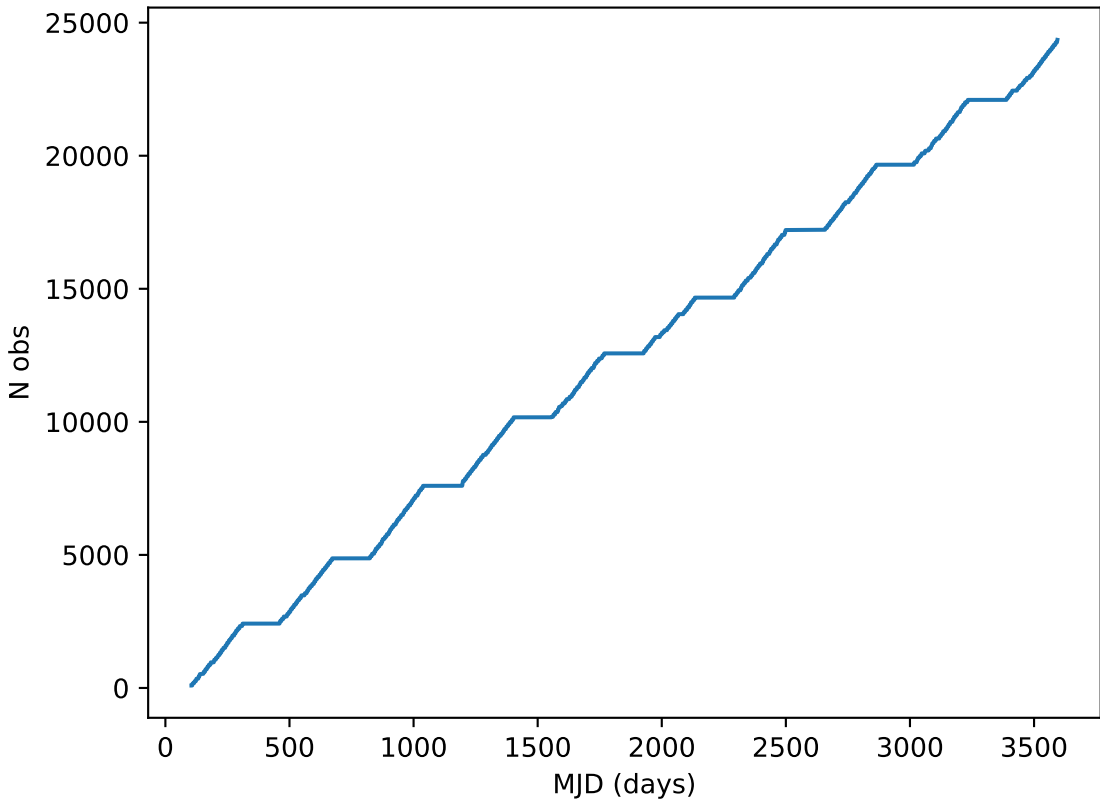
Imc_filter_balance_v3.4_10yrs all bands: DD:ECDFS Cumulative NVisits
