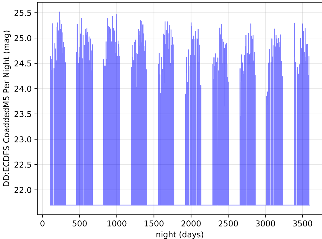
Imc_filter_balance_v3.4_10yrs z band: DD:ECDFS CoaddedM5 Per Night
