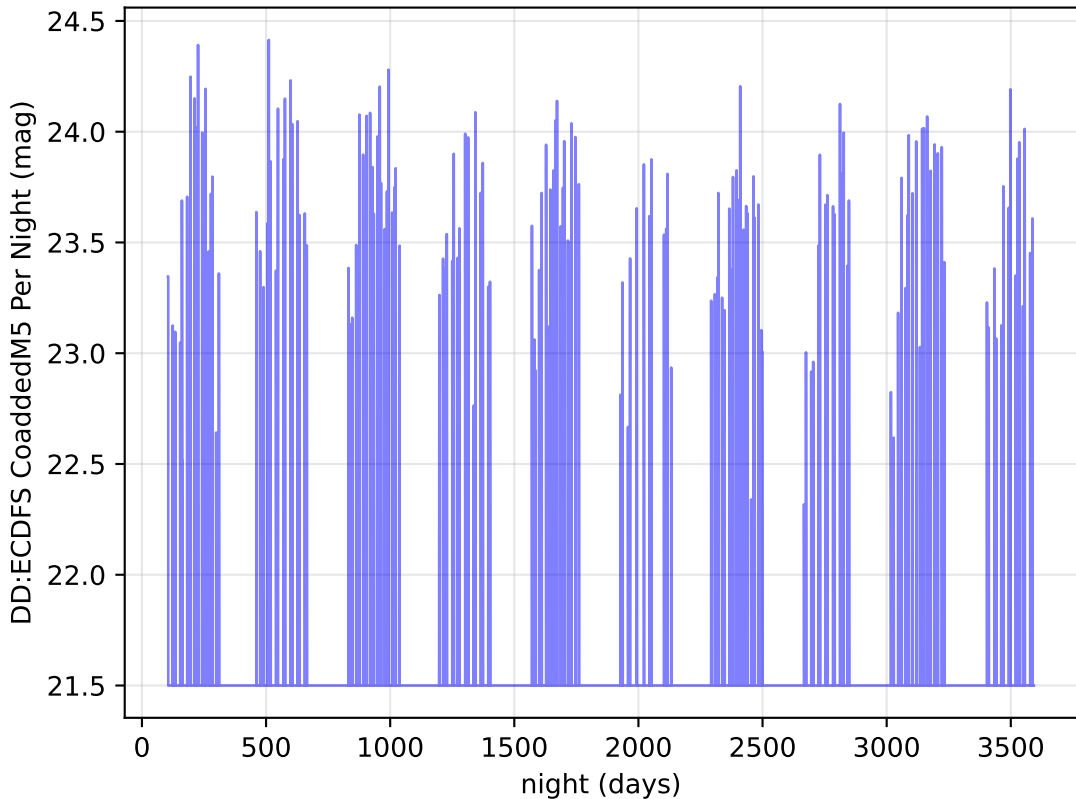
Imc_filter_balance_v3.4_10yrs y band: DD:ECDFS CoaddedM5 Per Night
