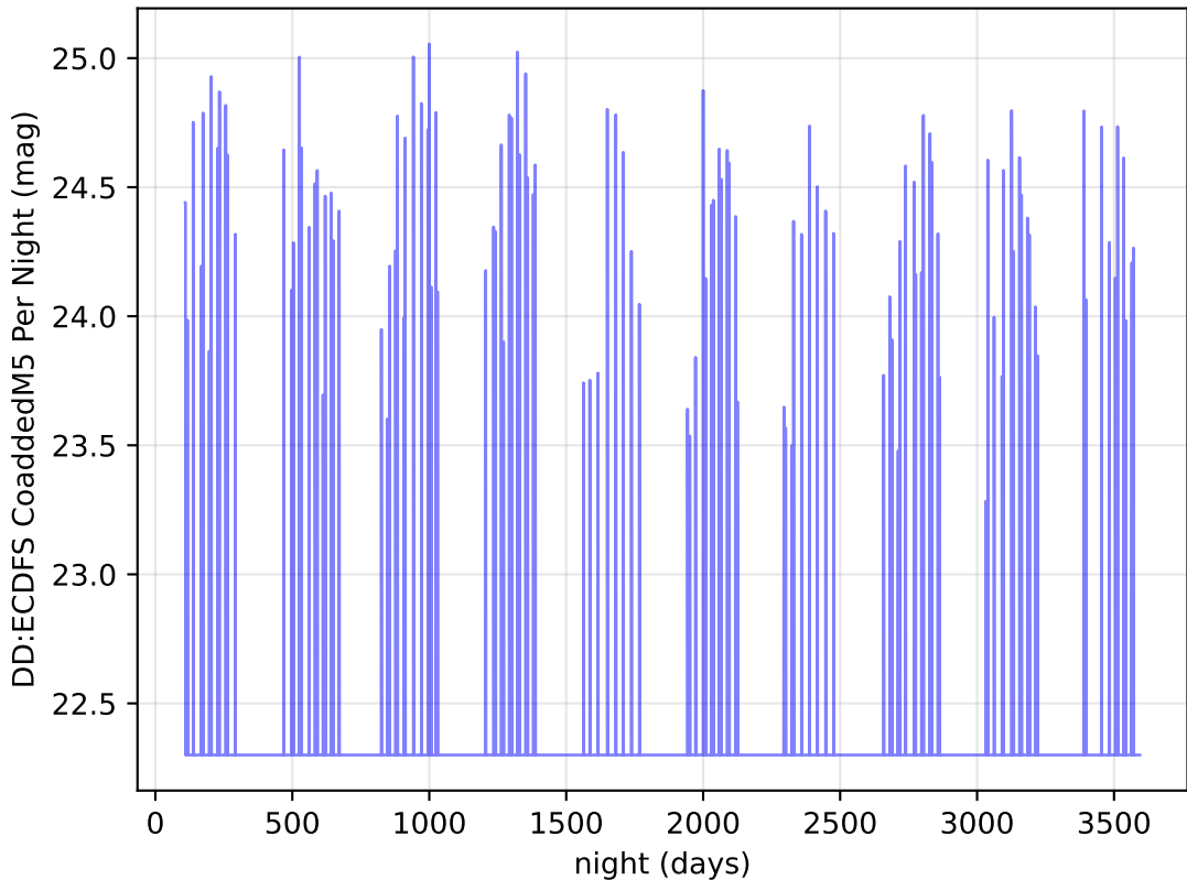
Imc_filter_balance_v3.4_10yrs u band: DD:ECDFS CoaddedM5 Per Night
