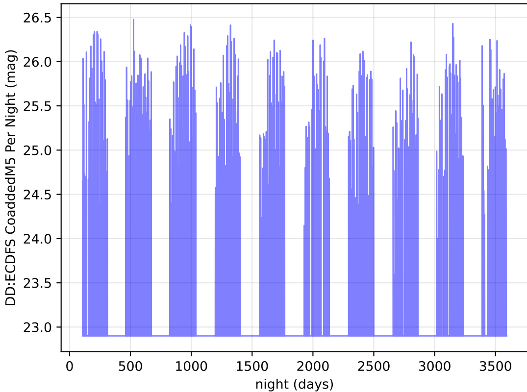
Imc_filter_balance_v3.4_10yrs r band: DD:ECDFS CoaddedM5 Per Night
