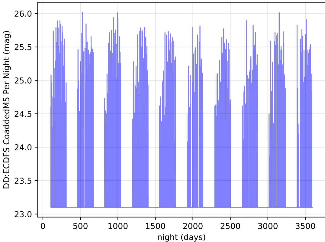
Imc_filter_balance_v3.4_10yrs i band: DD:ECDFS CoaddedM5 Per Night
