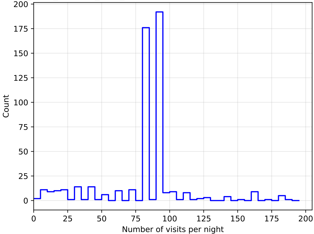
Imc_filter_balance_v3.4_10yrs all bands: DD: COSMOS NVisitsPerNight
