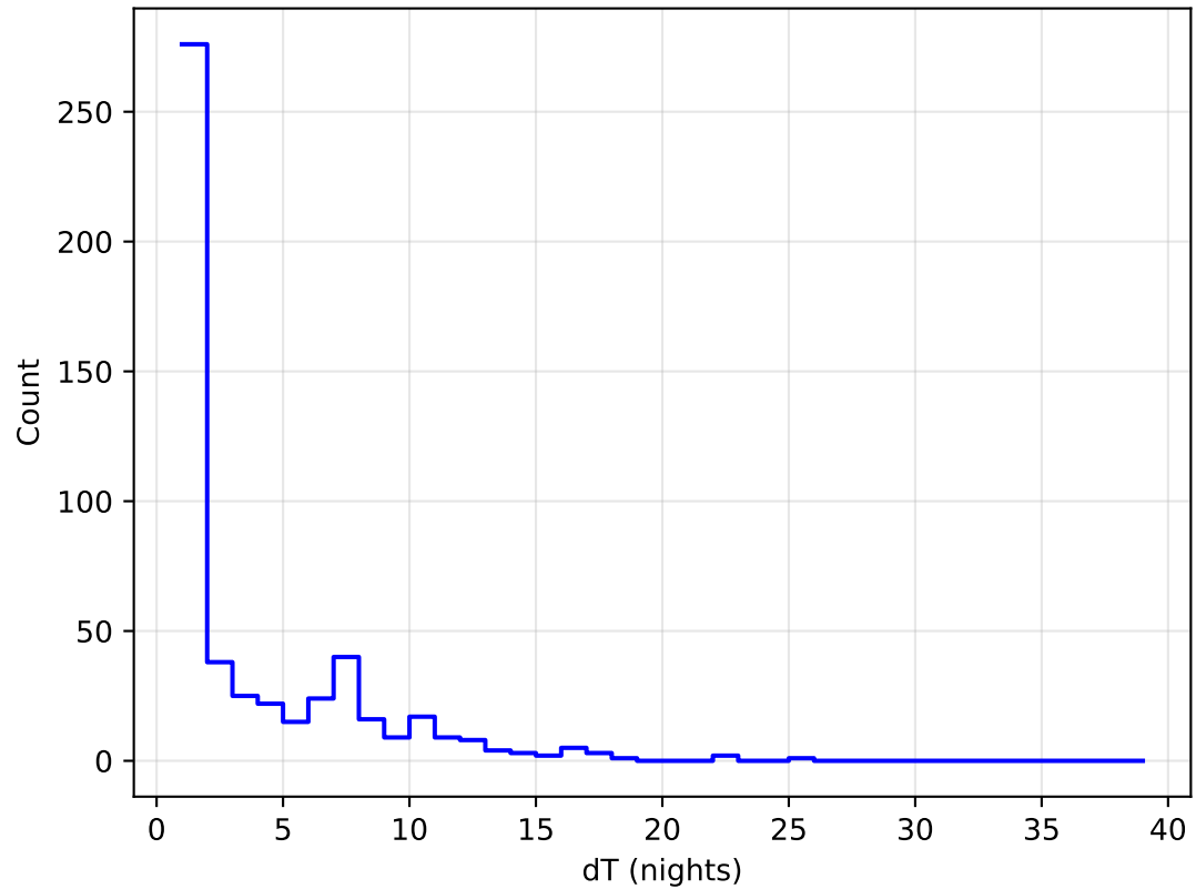
Imc_filter_balance_v3.4_10yrs all bands: DD: COSMOS Delta Nights Histogram
