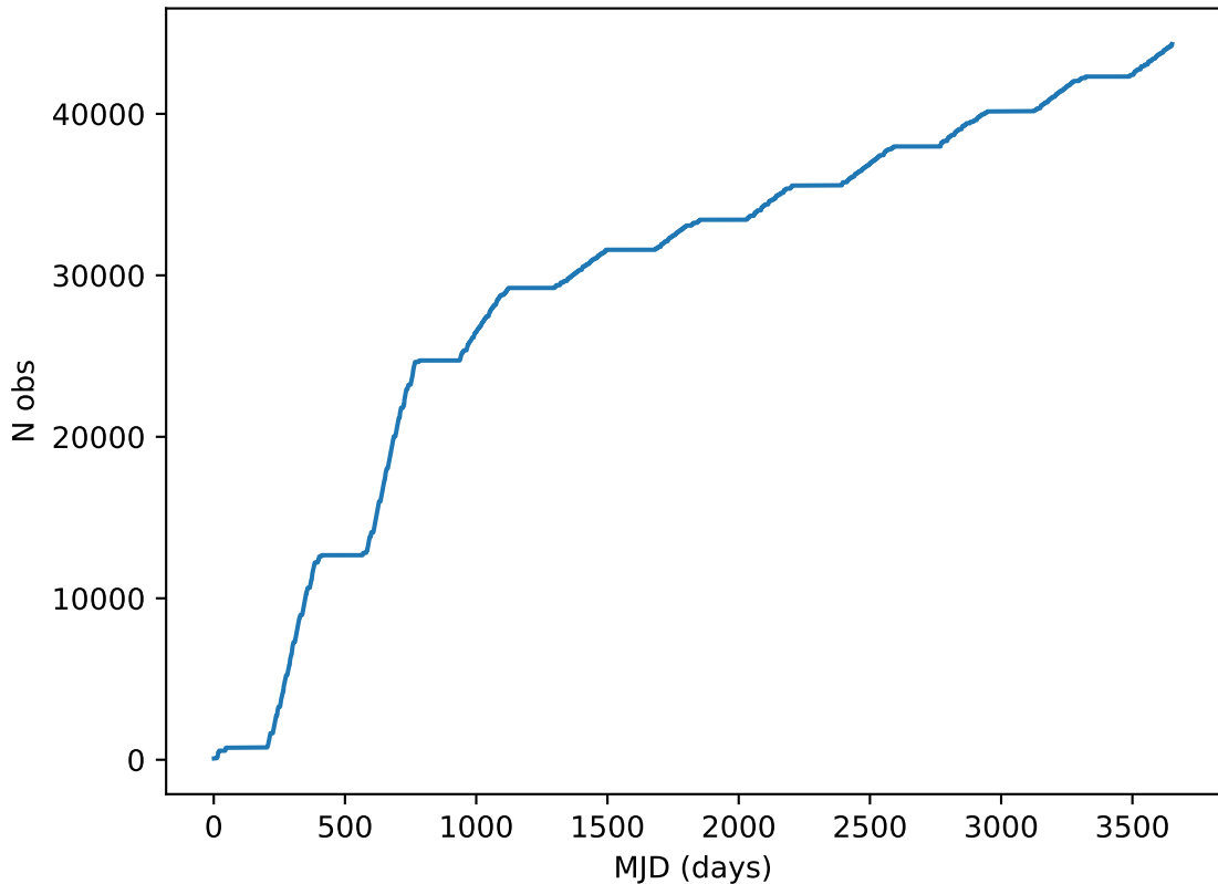
Imc_filter_balance_v3.4_10yrs all bands: DD: COSMOS Cumulative NVisits
