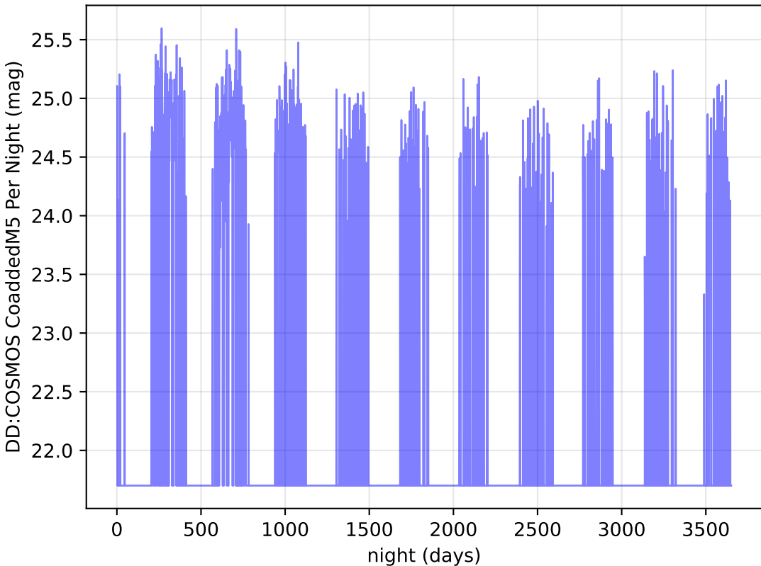
Imc_filter_balance_v3.4_10yrs z band: DD: COSMOS CoaddedM5 Per Night
