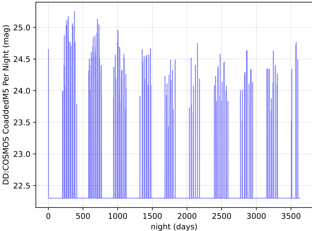
Imc_filter_balance_v3.4_10yrs u band: DD:COSMOS CoaddedM5 Per Night
