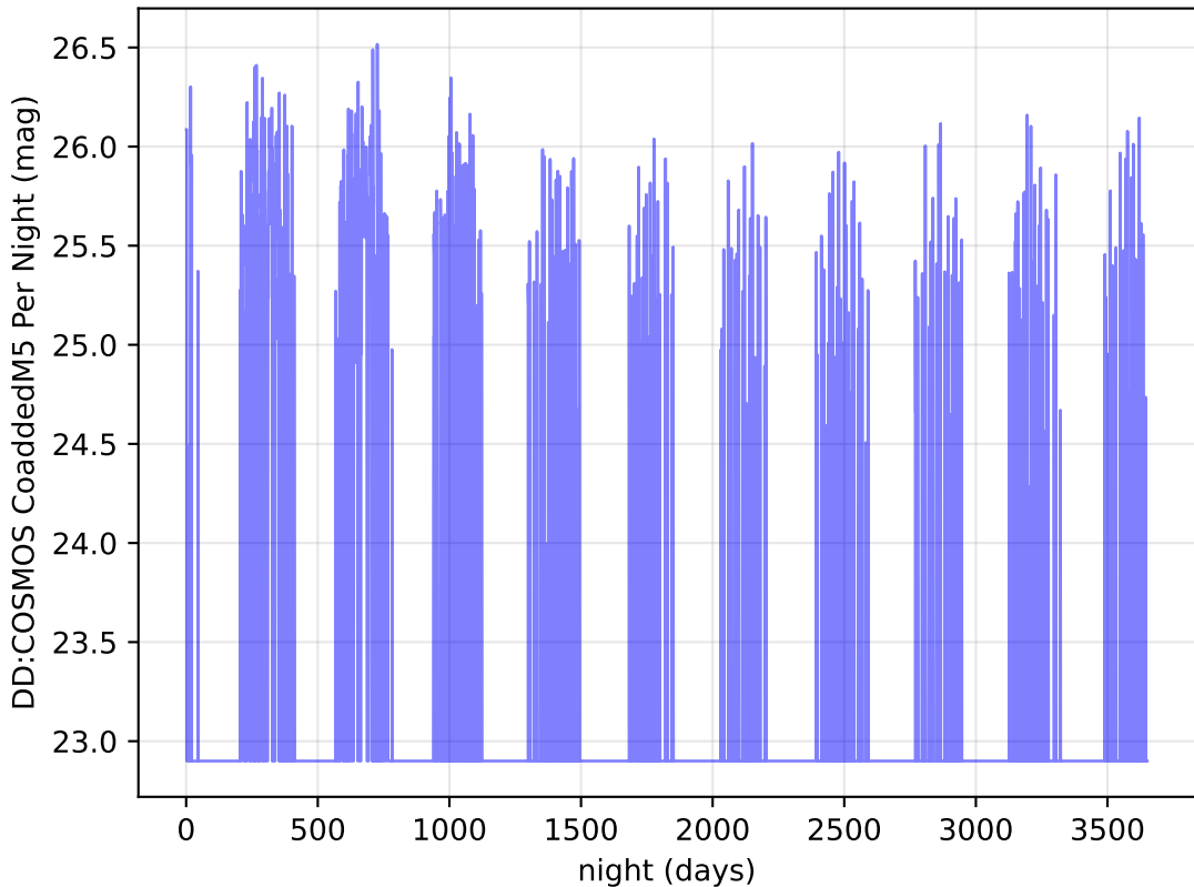
Imc_filter_balance_v3.4_10yrs r band: DD:COSMOS CoaddedM5 Per Night
