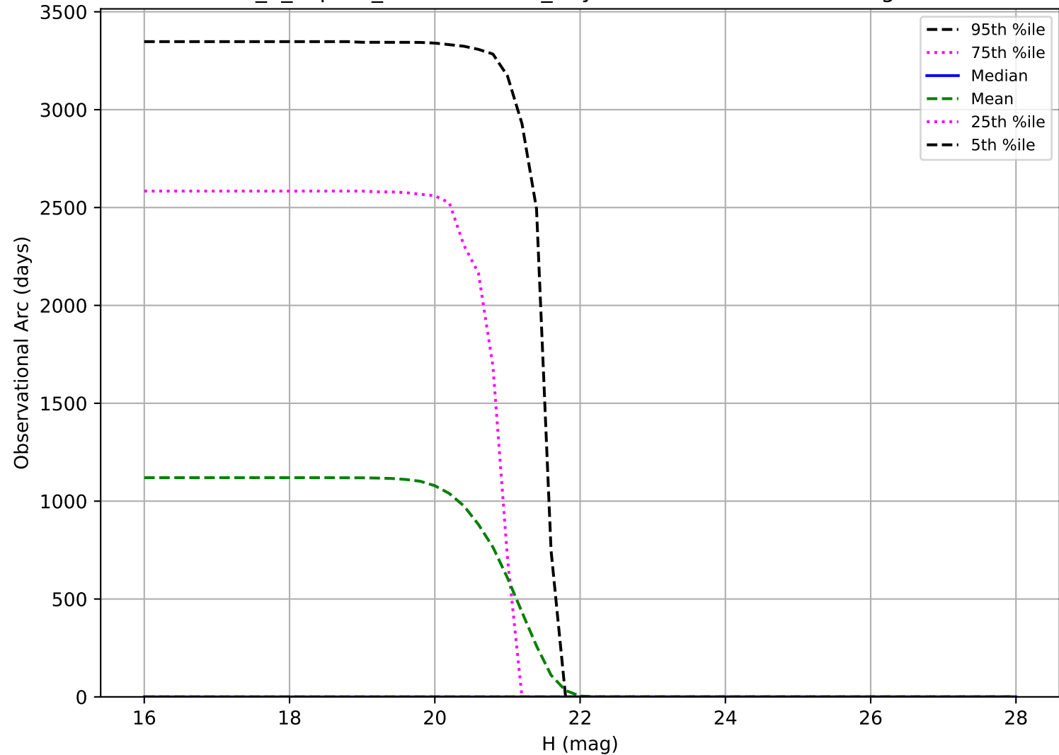
internal_u_expt60_nscale1.5v3.4_10yrs: Observational Arc Length Vatra
