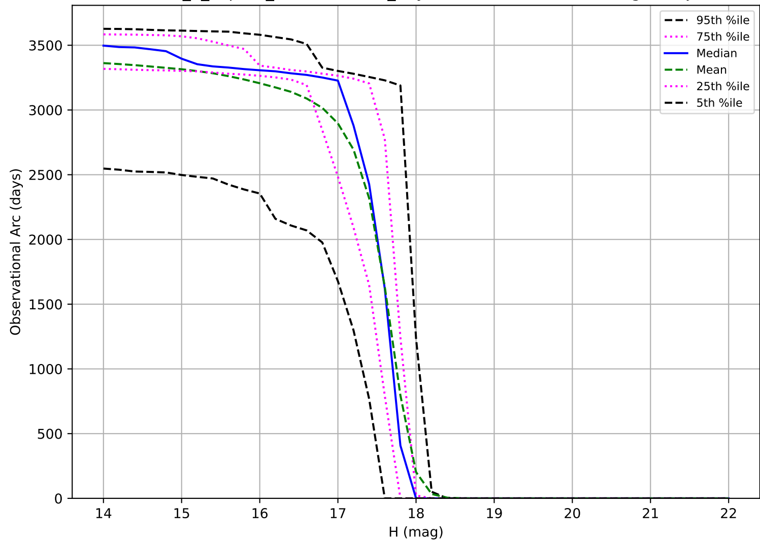
internal_u_expt60_nscale1.5v3.4_10yrs: Observational Arc Length Trojan
