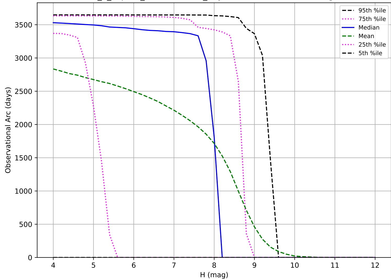
internal_u_expt60_nscale1.5v3.4_10yrs: Observational Arc Length TNO
