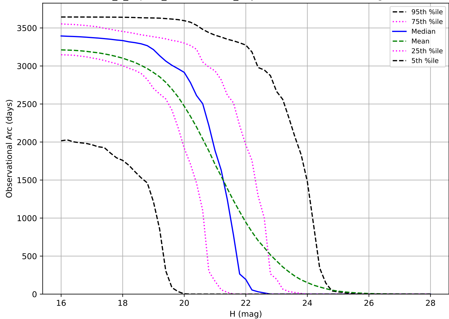
internal_u_expt60_nscale1.5v3.4_10yrs: Observational Arc Length PHA
