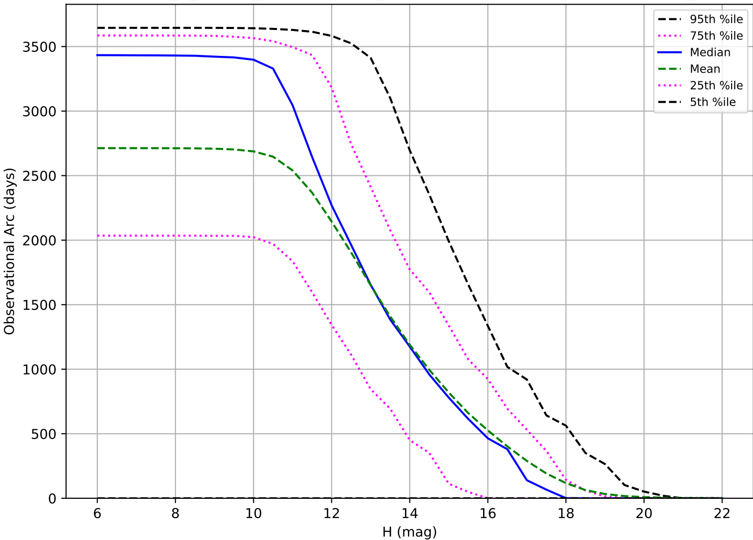
internal_u_expt60_nscale1.5v3.4_10yrs: Observational Arc Length OCC_r5
