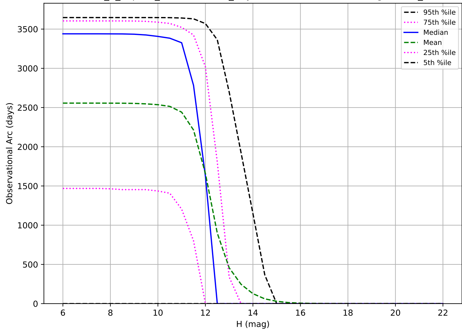
internal_u_expt60_nscale1.5v3.4_10yrs: Observational Arc Length OCC_r20
