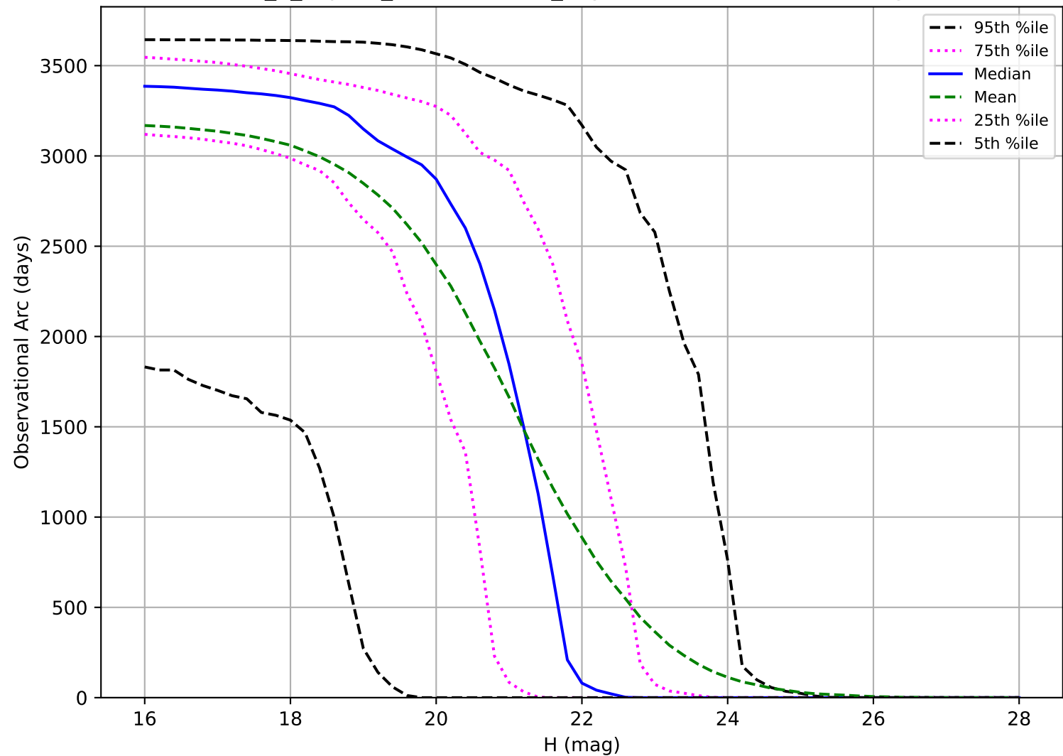
internal_u_expt60_nscale1.5v3.4_10yrs: Observational Arc Length NEO
