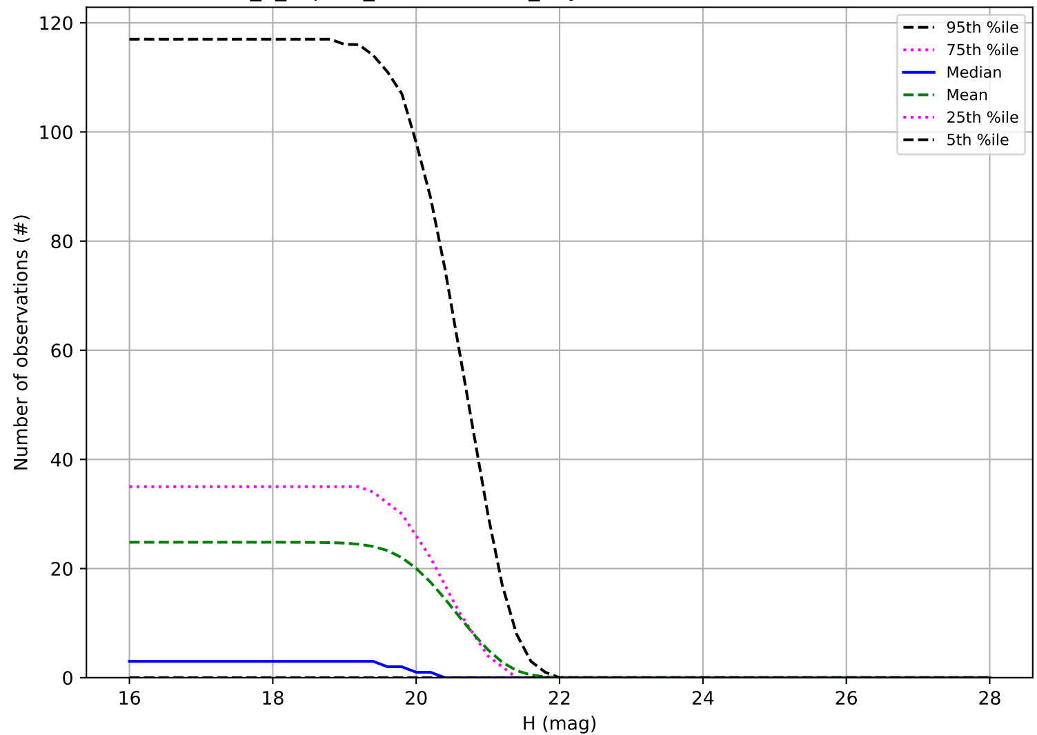
internal_u_expt60_nscale1.5v3.4_10yrs: Number of observations Vatira
