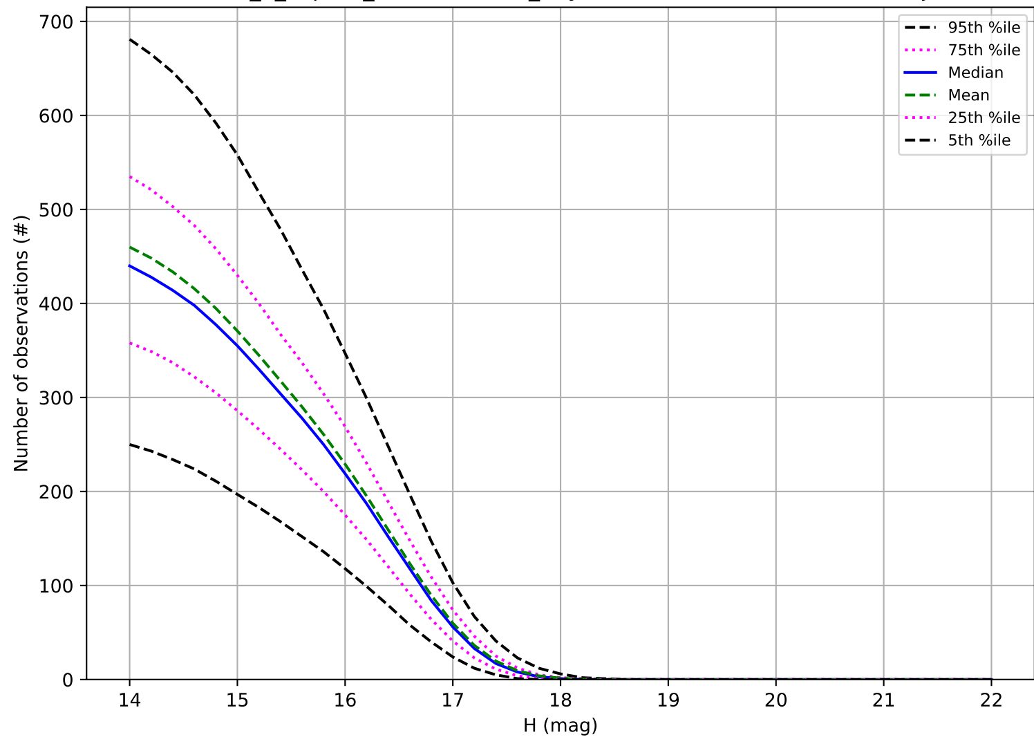
internal_u_expt60_nscale1.5v3.4_10yrs: Number of observations Trojan
