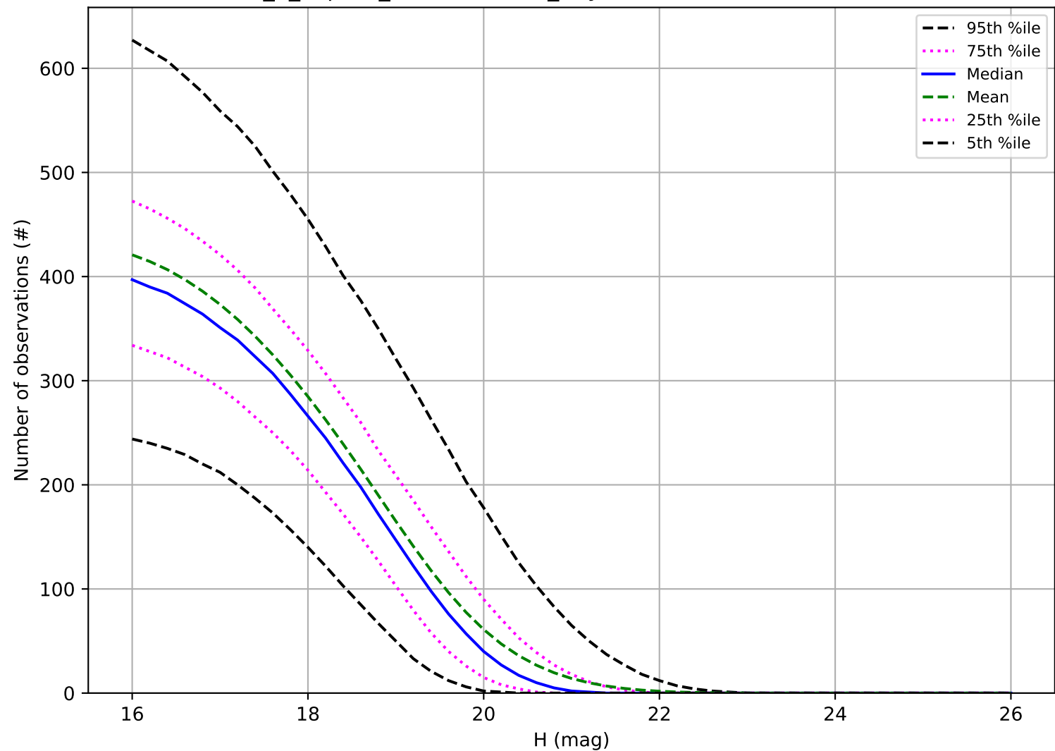
internal_u_expt60_nscale1.5v3.4_10yrs: Number of observations MBA
