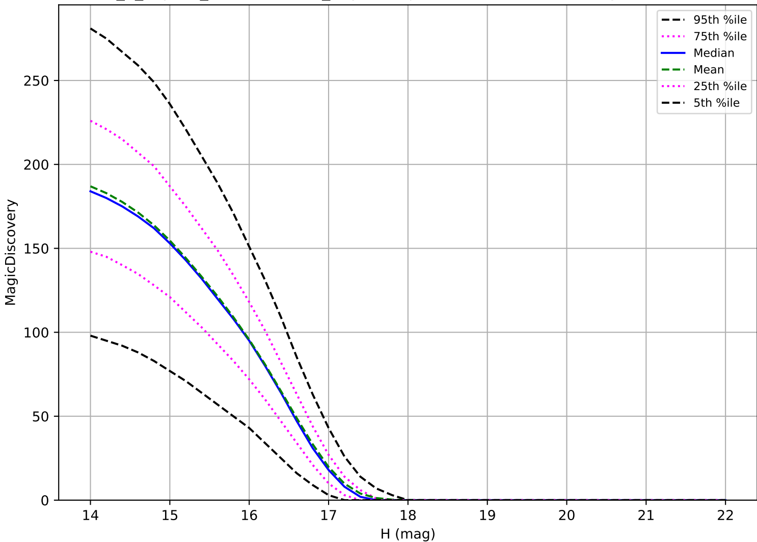
internal_u_expt60_nscale1.5v3.4_10yrs: Trojan 6 detections in 60 nights detection loss
