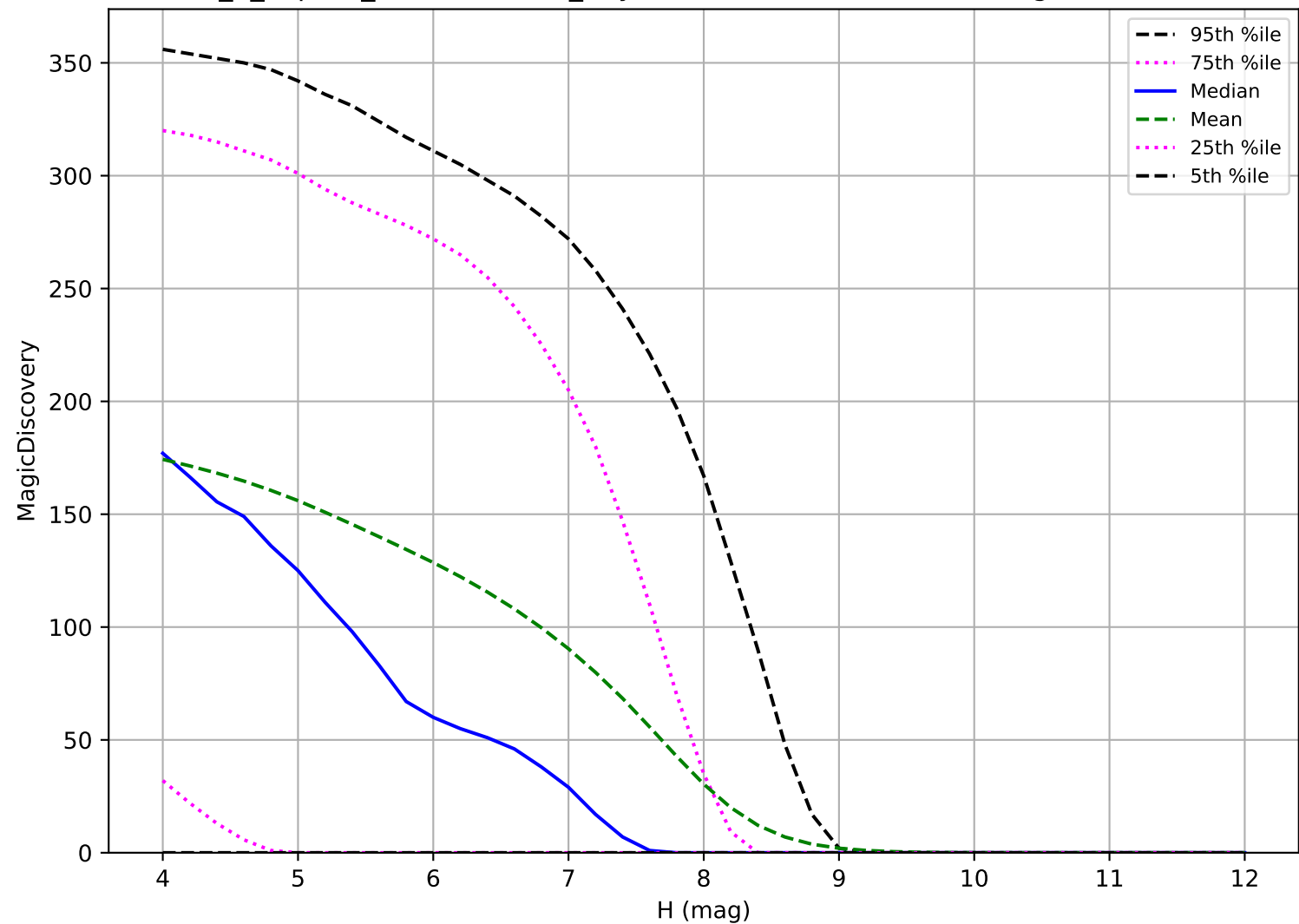
internal_u_expt60_nscale1.5v3.4_10yrs: TNO 6 detections in 60 nights detection loss
