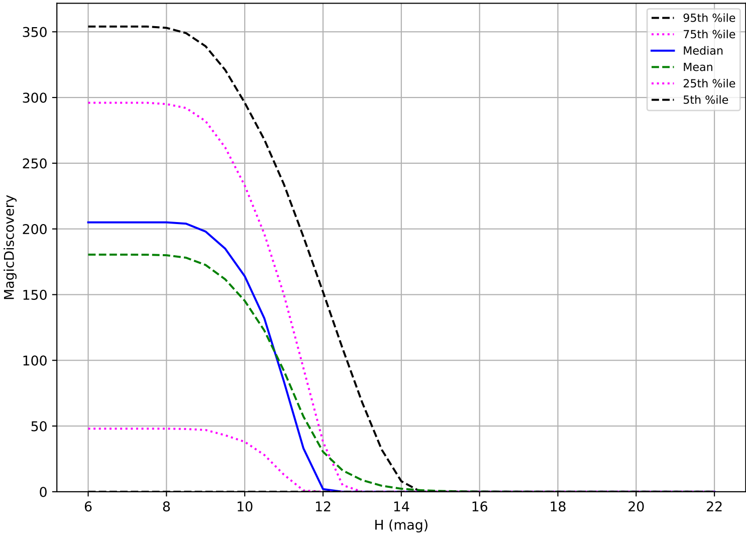
internal_u_expt60_nscale1.5v3.4_10yrs: OCC_r20 6 detections in 60 nights detection loss
