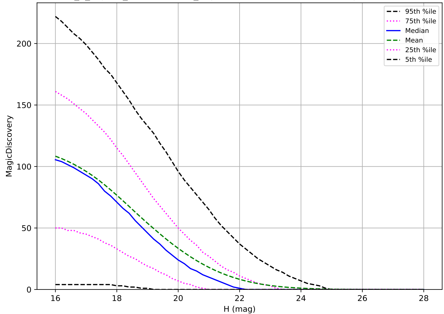
internal_u_expt60_nscale1.5v3.4_10yrs: NEO 6 detections in 60 nights detection loss
