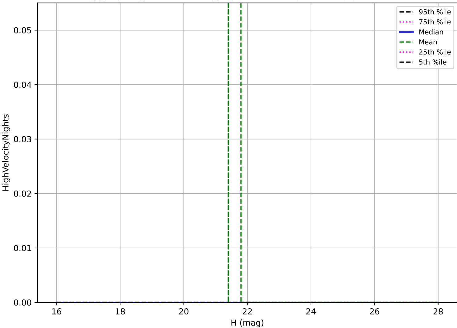
internal_u_expt60_nscale1.5v3.4_10yrs: Vatira High velocity pair detection loss
