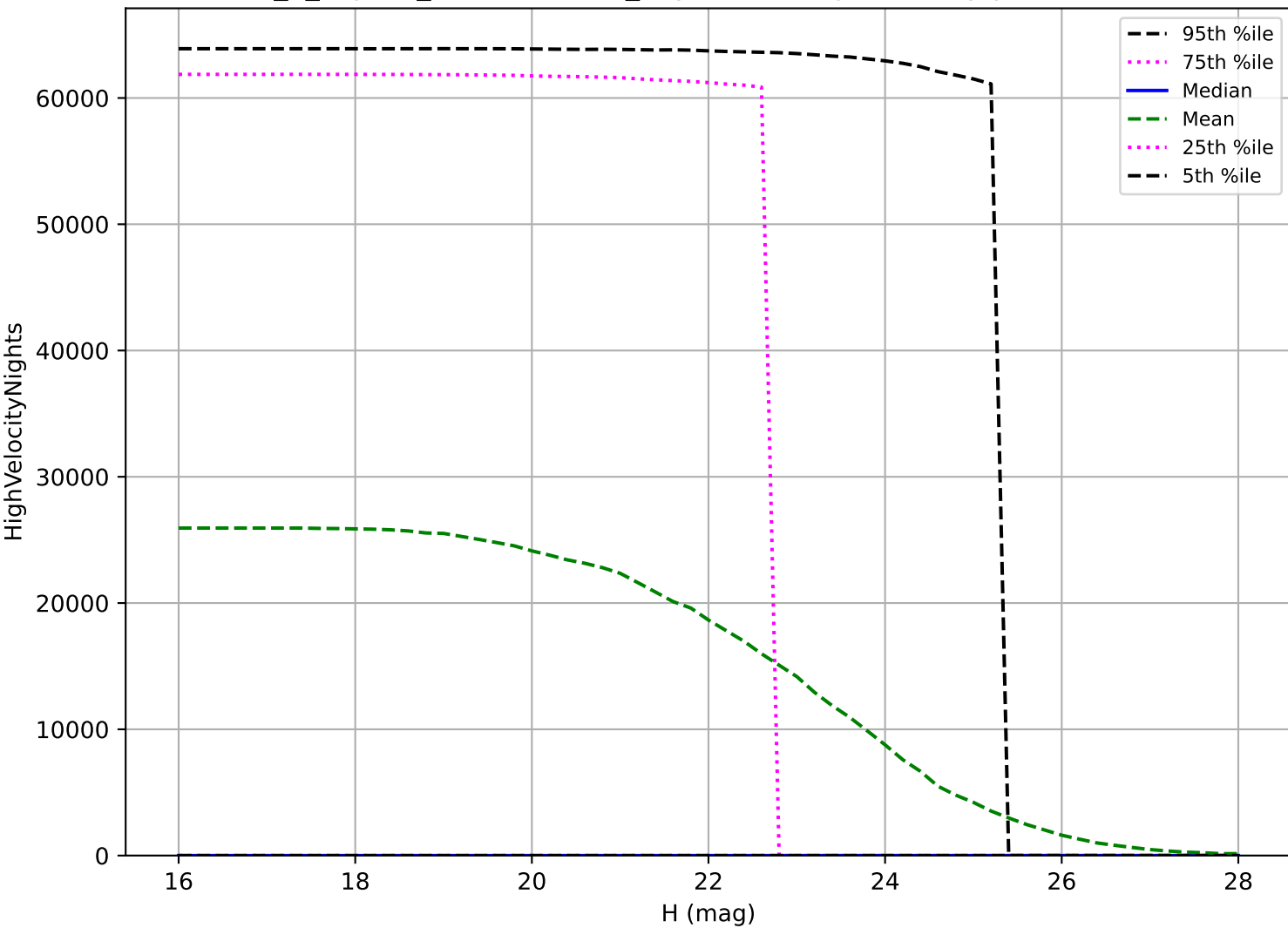
internal_u_expt60_nscale1.5v3.4_10yrs: PHA High velocity pair detection loss
