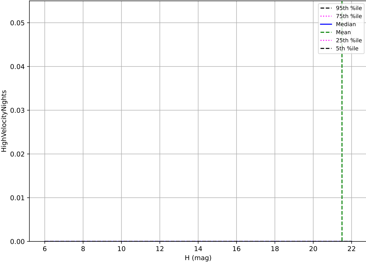
internal_u_expt60_nscale1.5v3.4_10yrs: OCC_r20 High velocity pair detection loss
