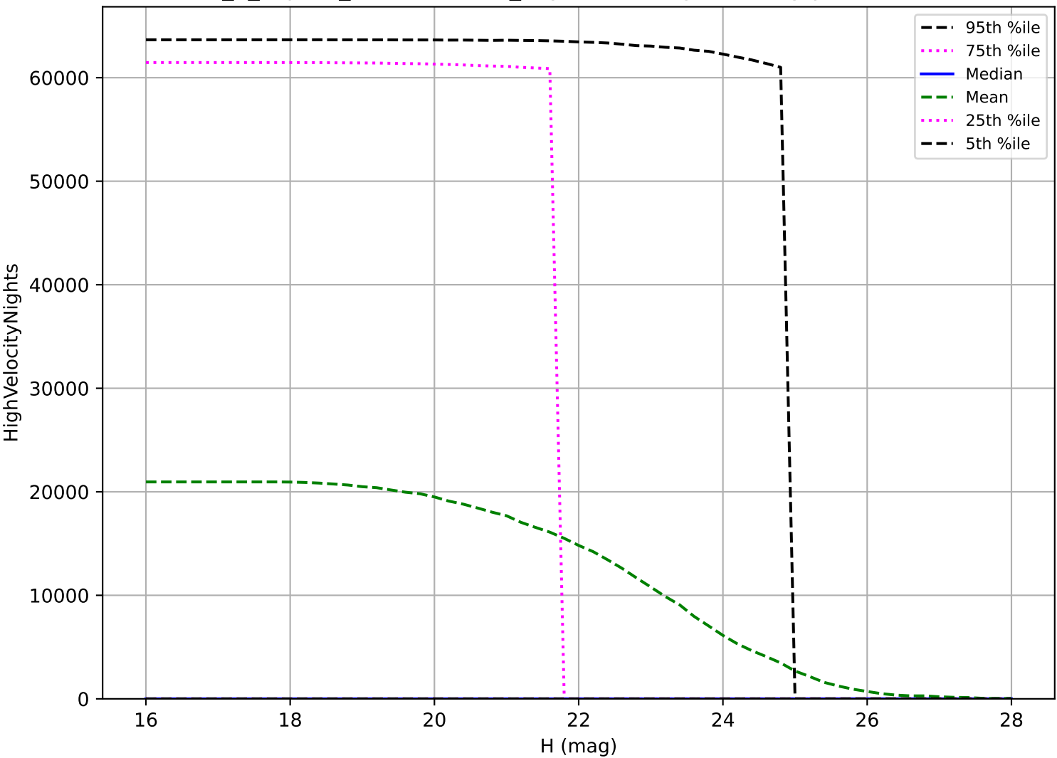
internal_u_expt60_nscale1.5v3.4_10yrs: NEO High velocity pair detection loss
