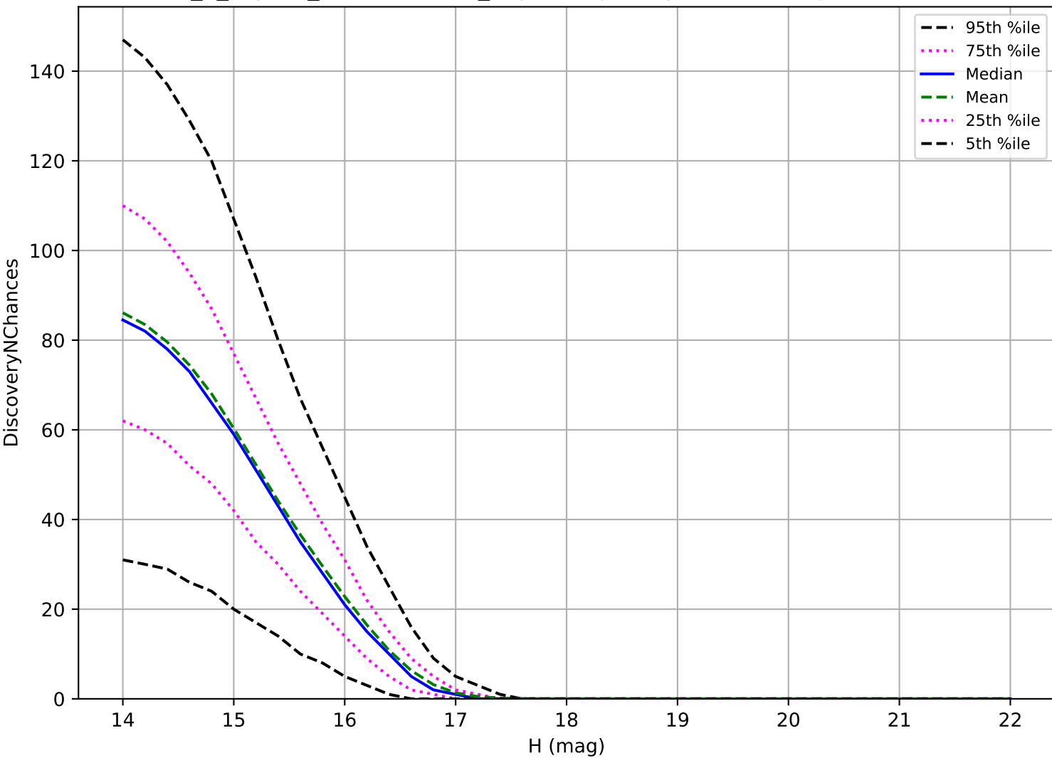
internal_u_expt60_nscale1.5v3.4_10yrs: Trojan 3 pairs in 15 nights detection loss
