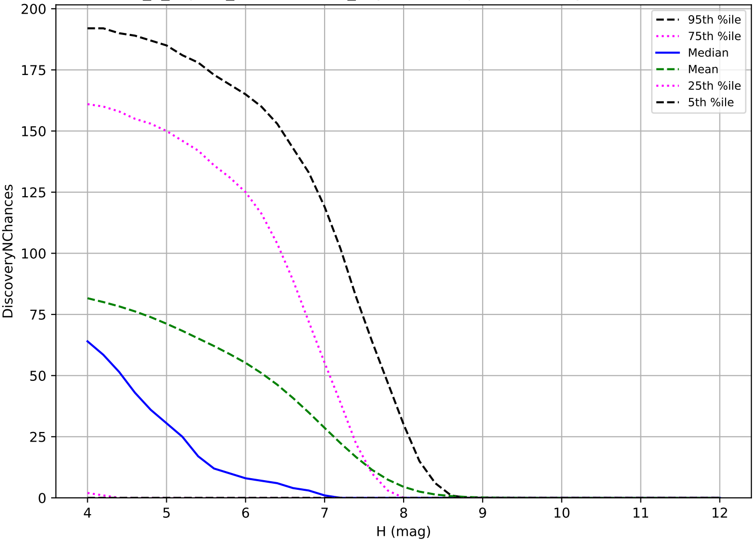
internal_u_expt60_nscale1.5v3.4_10yrs: TNO 3 pairs in 15 nights detection loss
