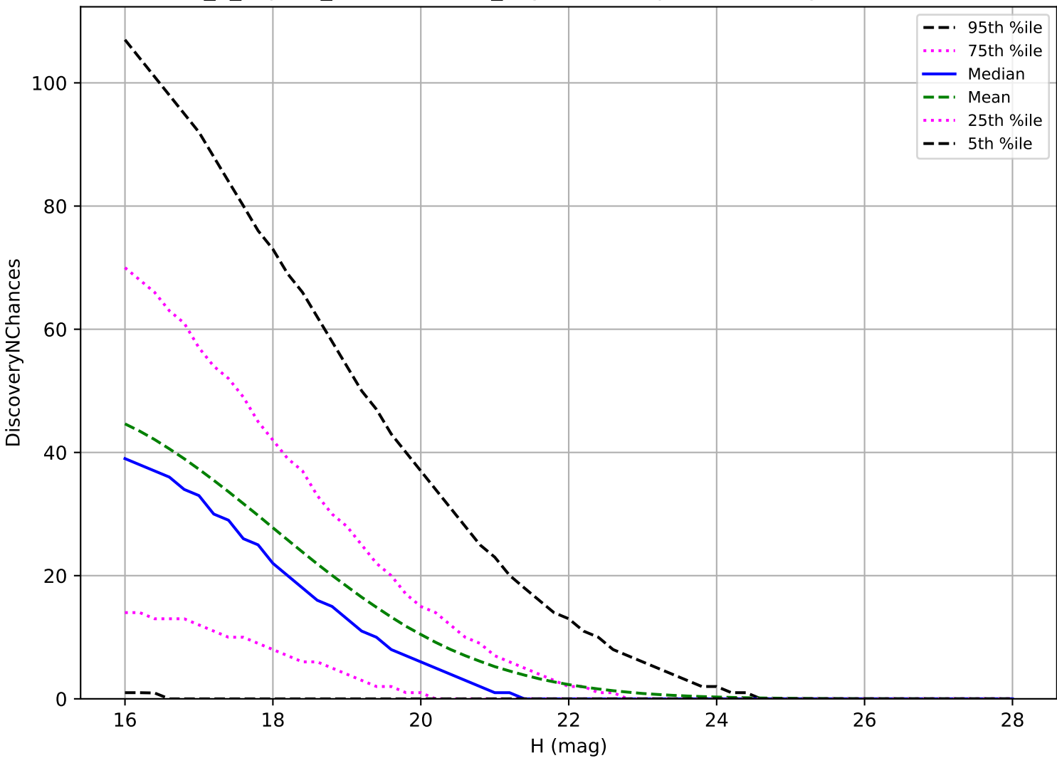
internal_u_expt60_nscale1.5v3.4_10yrs: PHA 3 pairs in 15 nights detection loss
