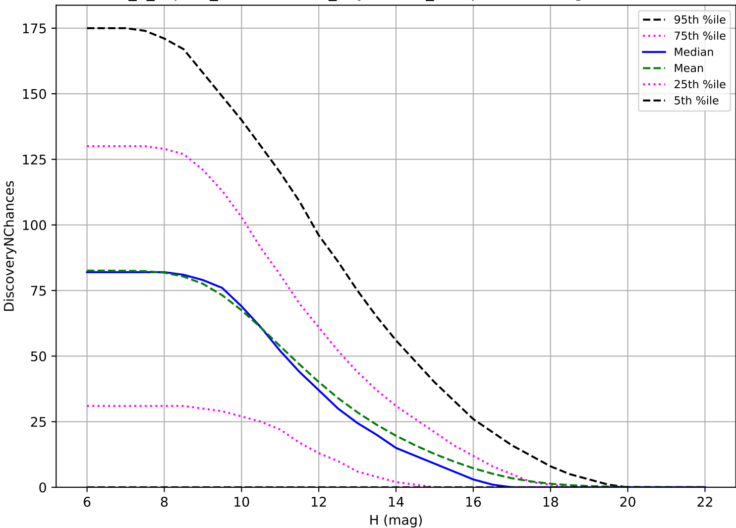
internal_u_expt60_nscale1.5v3.4_10yrs: OCC_r5 3 pairs in 15 nights detection loss
