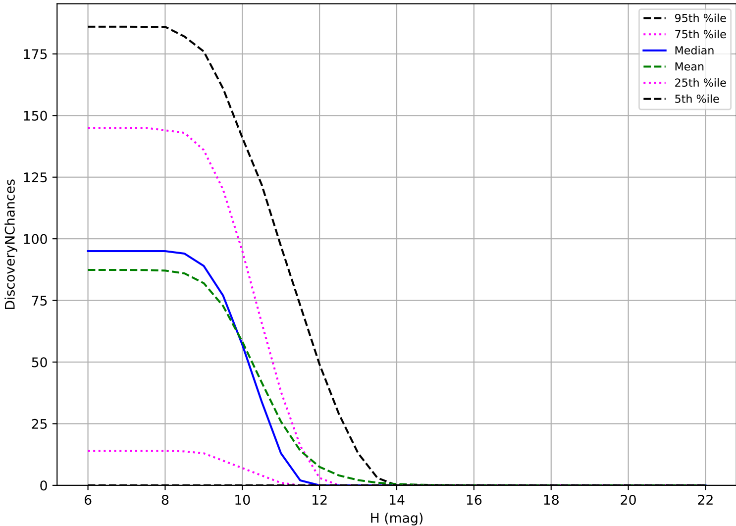
internal_u_expt60_nscale1.5v3.4_10yrs: OCC_r20 3 pairs in 15 nights detection loss
