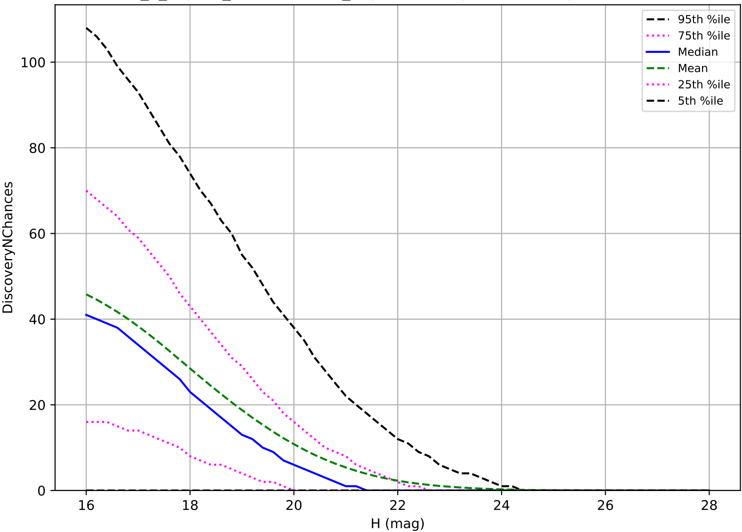
internal_u_expt60_nscale1.5v3.4_10yrs: NEO 3 pairs in 15 nights detection loss
