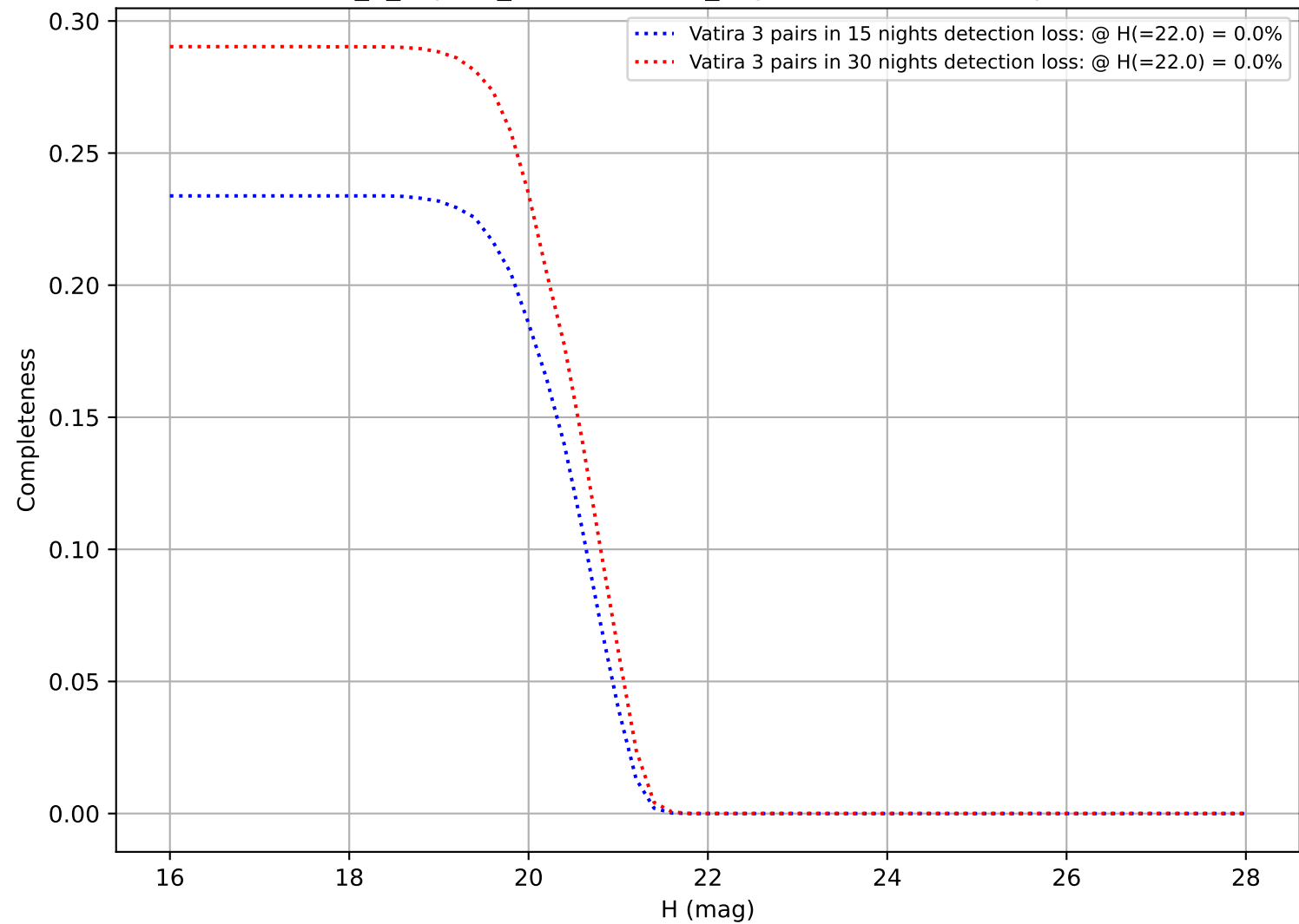
internal_u_expt60_nscale1.5v3.4_10yrs: DifferentialCompleteness
