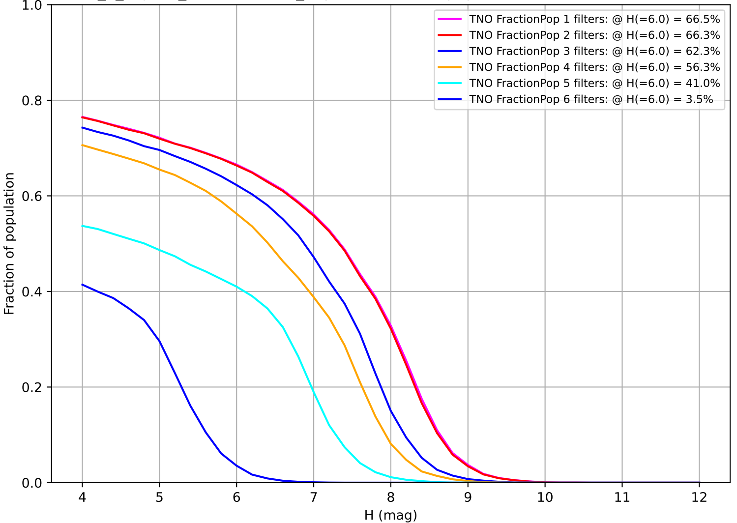
internal_u_expt60_nscale1.5v3.4_10yrs: Fraction of population with colors in X filters TNO
