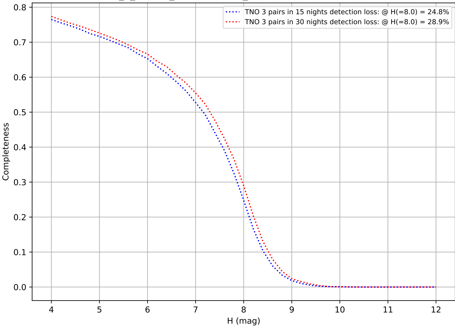
internal_u_expt60_nscale1.5v3.4_10yrs: DifferentialCompleteness
