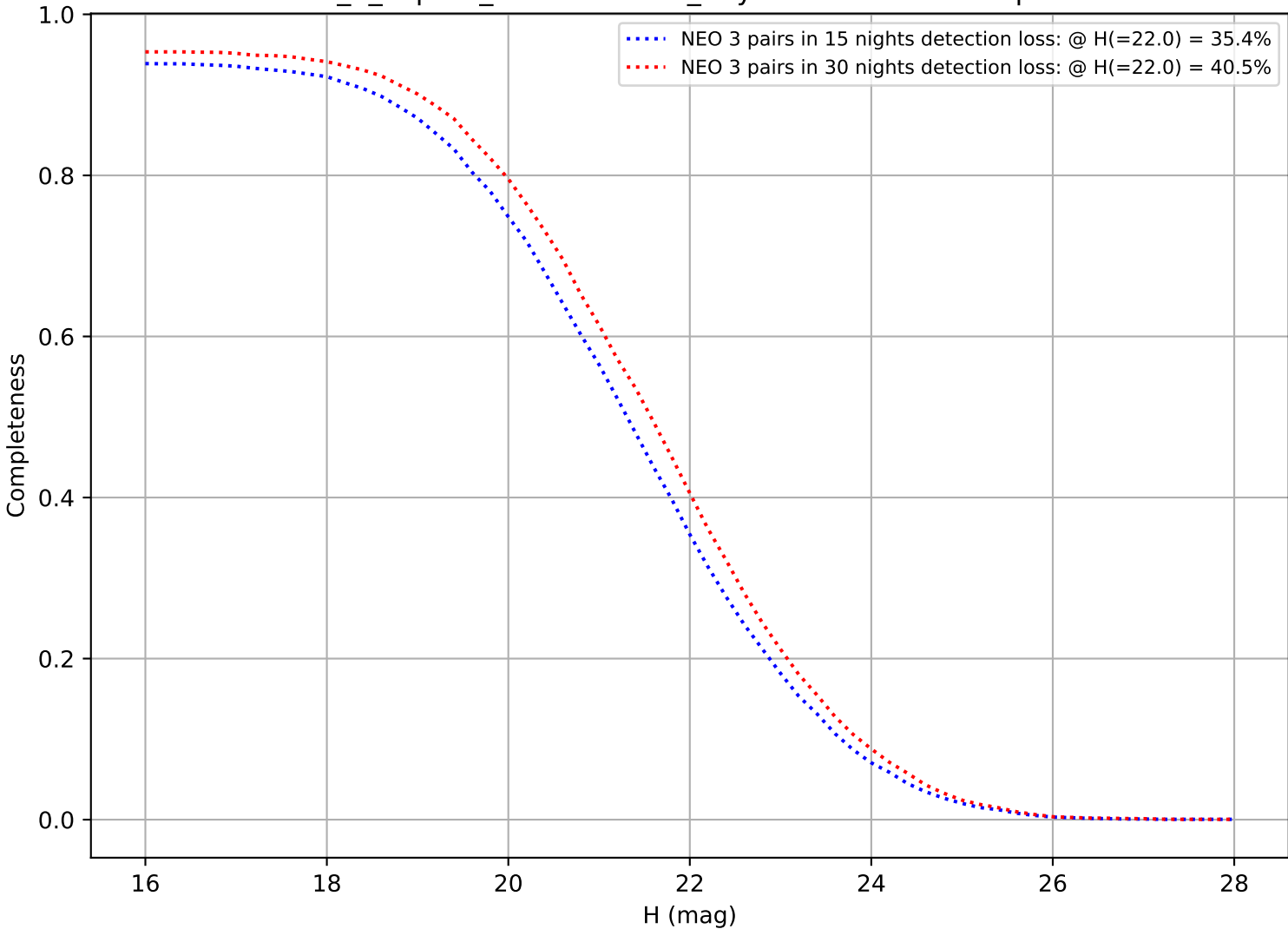
internal_u_expt60_nscale1.5v3.4_10yrs: DifferentialCompleteness
