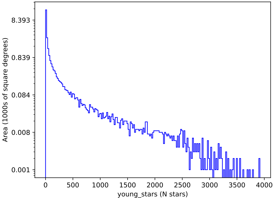
internal_u_expt60_nscale1.5v3.4_10yrs : young_stars
