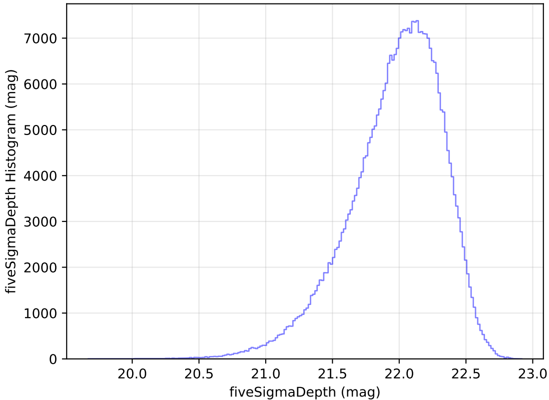
internal_u_expt60_nscale1.5v3.4_10yrs y: fiveSigmaDepth Histogram
