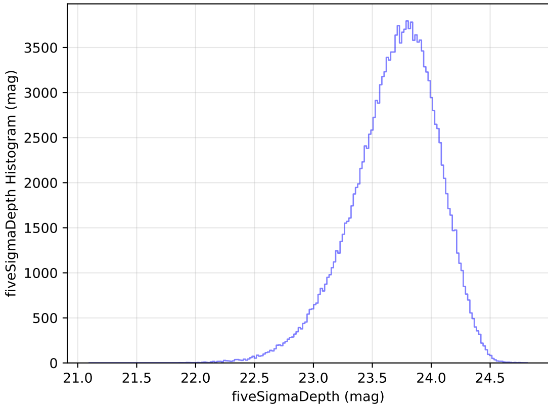
internal_u_expt60_nscale1.5v3.4_10yrs u: fiveSigmaDepth Histogram
