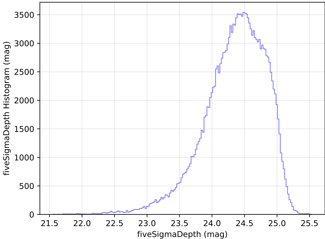
internal_u_expt60_nscale1.5v3.4_10yrs g: fiveSigmaDepth Histogram
